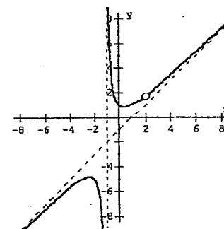
f(x) = \frac{(x^2 + 1)(x - 2)}{(x + 1)(x - 2)} Rational
