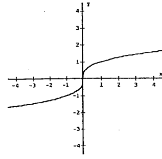
f(x) = \sqrt[3]{x} Cube Root
