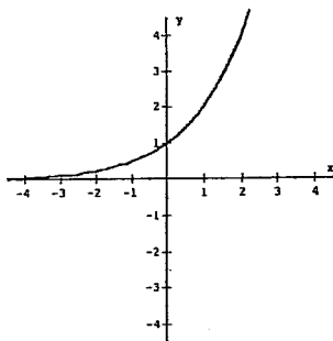
f(x) = a^x Exponential
